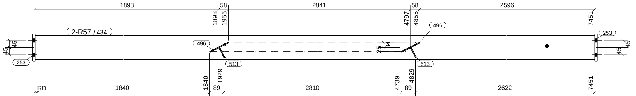
TOP VIEW
