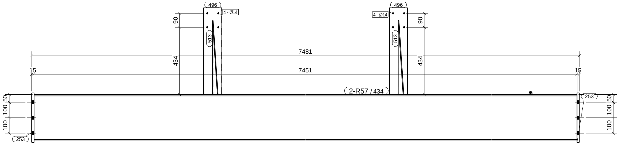
FRONT VIEW
